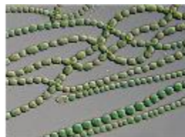
Blue-green algae
